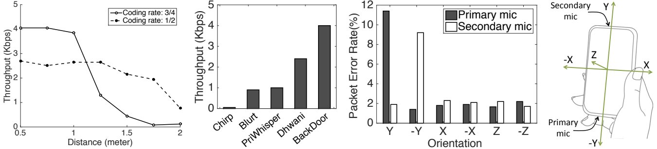
Figure 17: BackDoor Communication Results: (a) Throughput vs. Distance, (b) Throughput comparison against related P2P communication schemes. (c) Packet error rate vs. Orientation. (d) Phone orientations.
