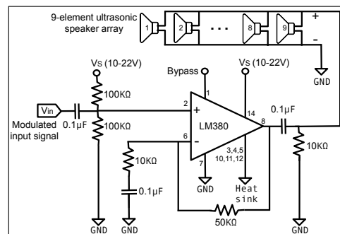
Figure 16: The circuit diagram of the jamming transmitter.
