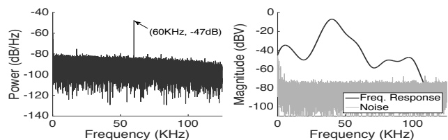
Figure 4: (a) Microphone signals (measured before the LPF) confirm the diaphragm and pre-amplifier’s sensitivity to ultrasound frequencies. (b) Full freq. response at the output of the amplifier.
