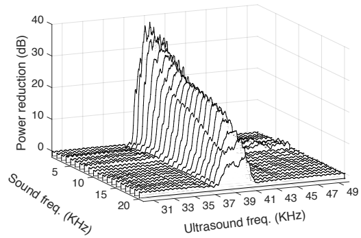
Figure 13: The reduction in sound power due to the AGC: reduction maximum for the 40\text{kHz} tone due to the speaker's resonance at this frequency.
