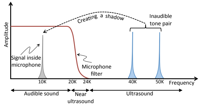
Figure 1: The main idea underlying BackDoor .
